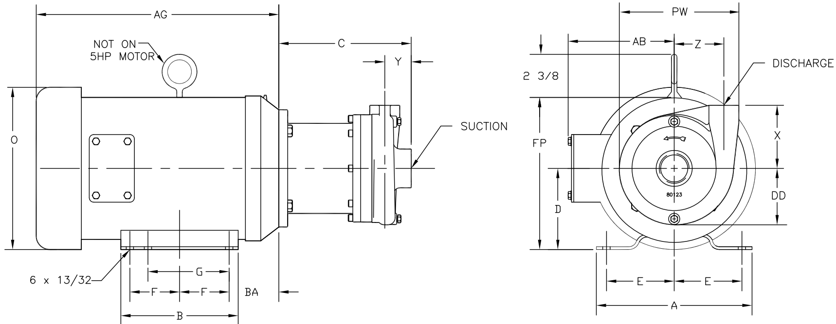
PUMP END DIMENSIONS
