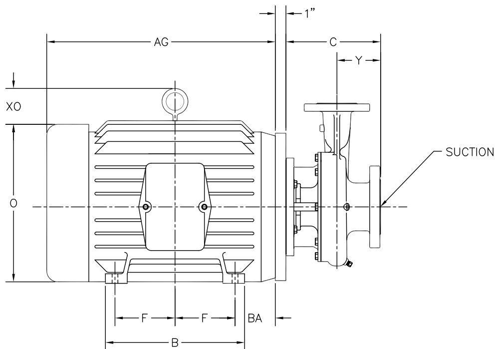
MOTOR END DIMENSIONS
