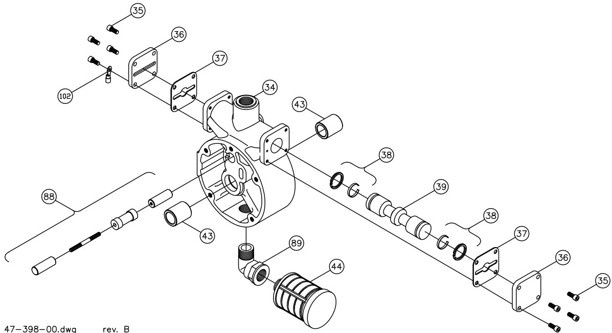
47-398-00.dwg rev. B
