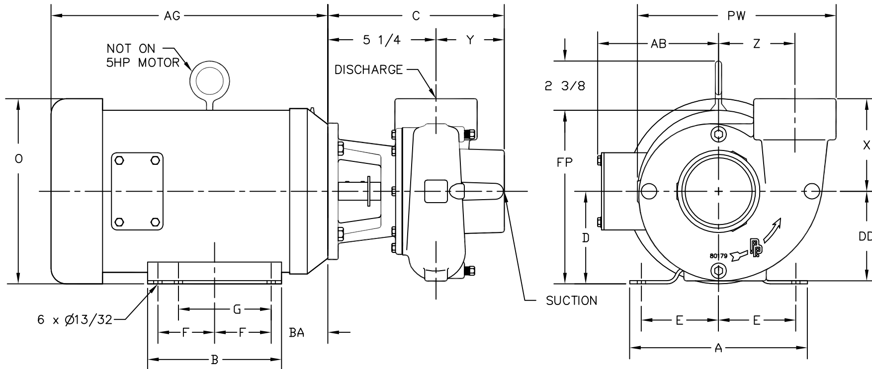
PUMP END DIMENSIONS
